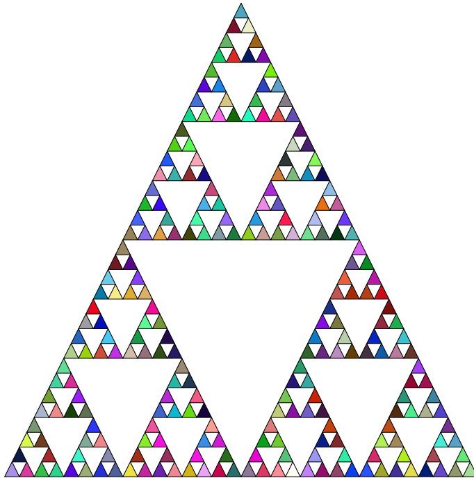
Figure 33: Using Transformations
