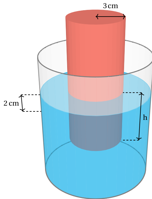
Figure 30: Solid cylinder immersed in water
