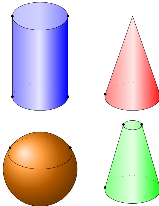
Figure 11: Points of tangency
