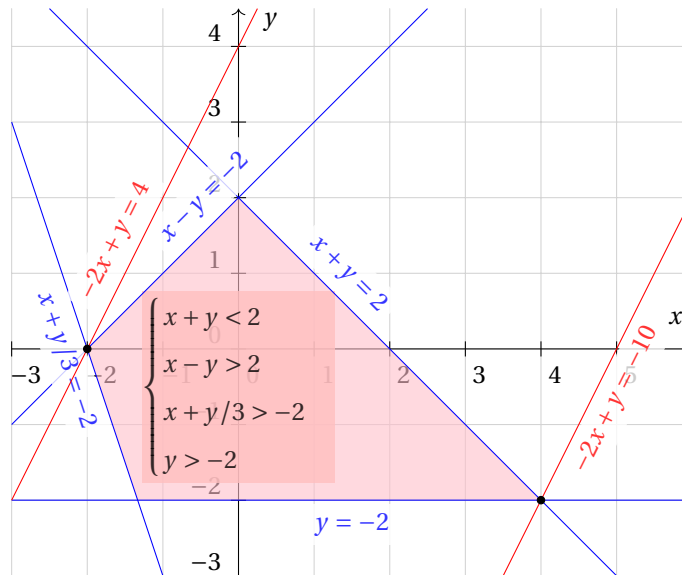
Figure 37: The g:DlinprogRegion() method
