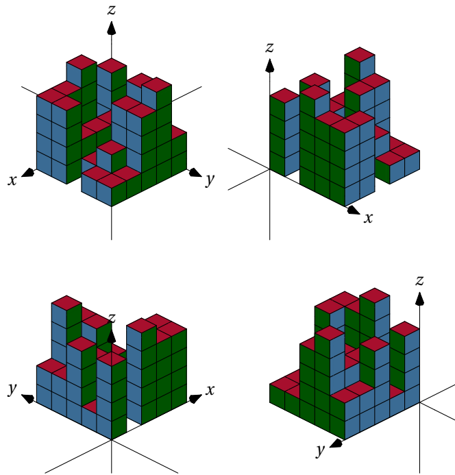
Figure 40: Stack of Cubes
