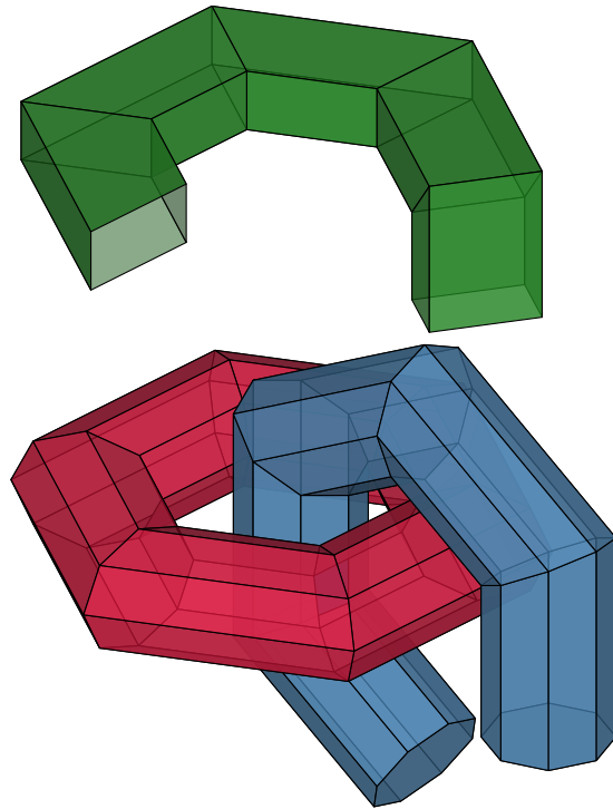
Figure 22: Example with line2tube and section2tube
