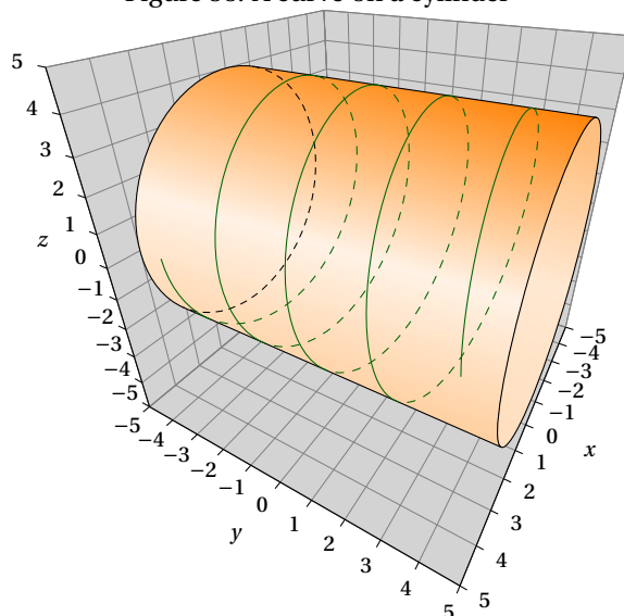
Figure 38: A curve on a cylinder
