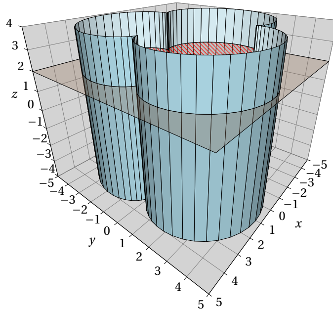
Figure 21: Section of a non-circular cylinder
