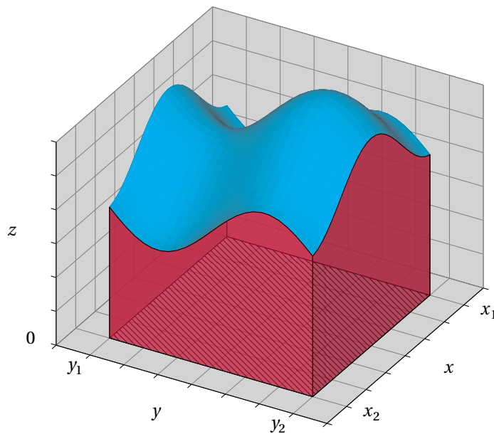
Figure 42: Volume corresponding to \int_{x_1}^{x_2} \int_{y_1}^{y_2} f(x,y) dx dy
