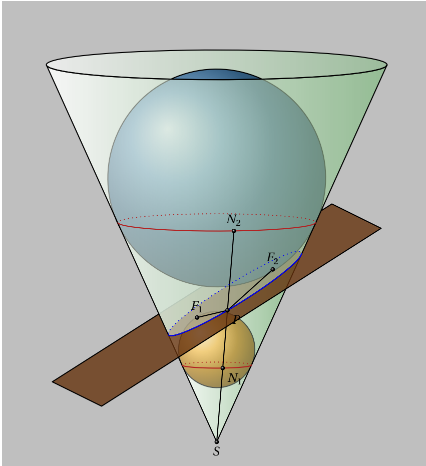
Figure 41: Illustration of Dandelin's Theorem
