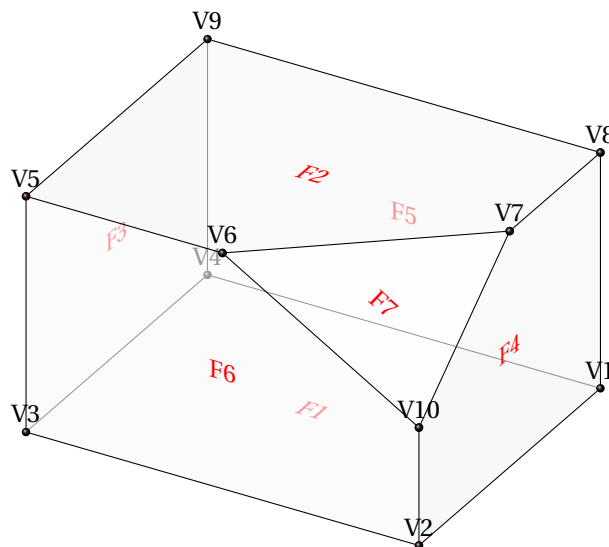
Figure 13: Visualize the faces and vertices of a polyhedron
