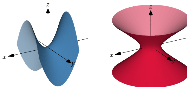
Figure 19: Surfaces using the addwall option
