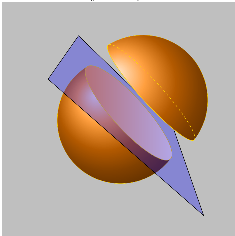
Figure 10: Cut sphere
