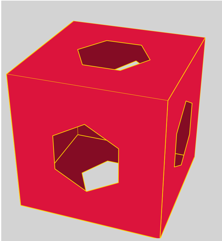
Figure 36: Faces of a cube with holes in it and a regular hexagon
