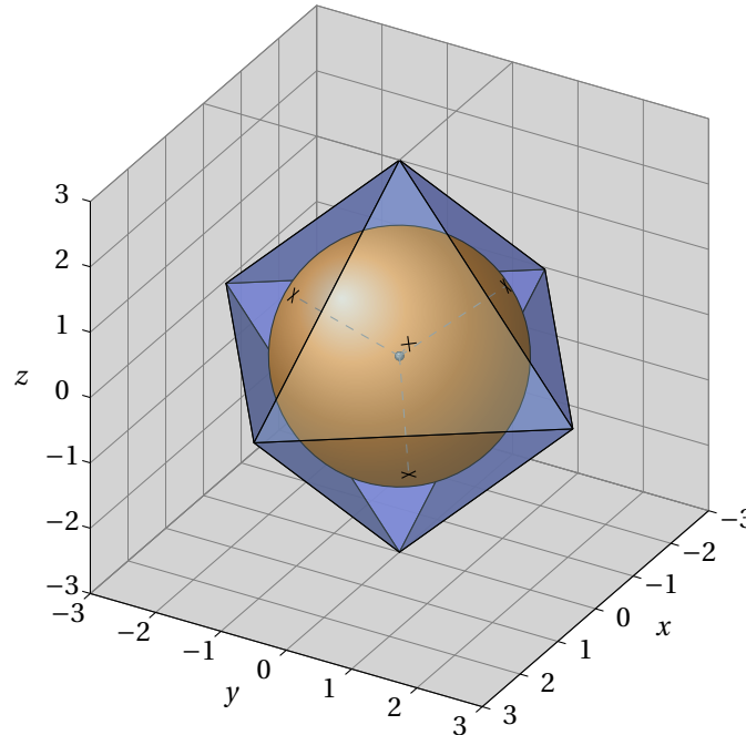
Figure 26: Sphere inscribed in an octahedron with the center projected onto the faces
