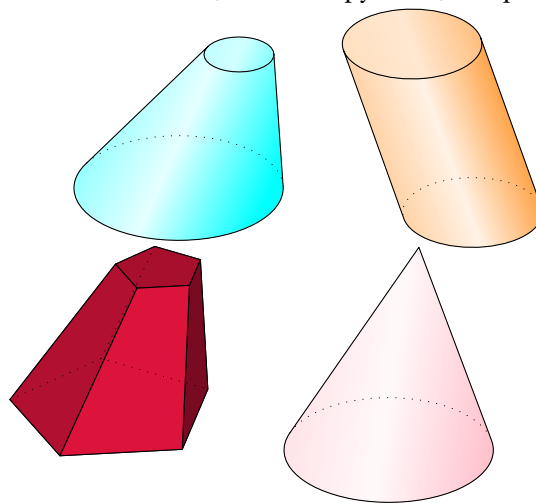
Figure 14: Truncated cone, truncated pyramid, oblique cylinder
