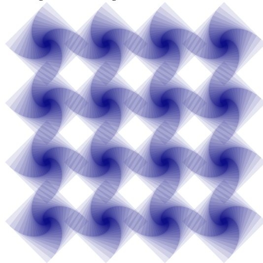
Figure 35: Using Shift, Rotate and Scale
