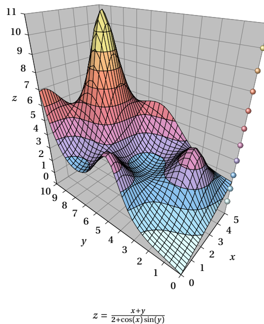
Figure 18: Example of contour lines on a surface
