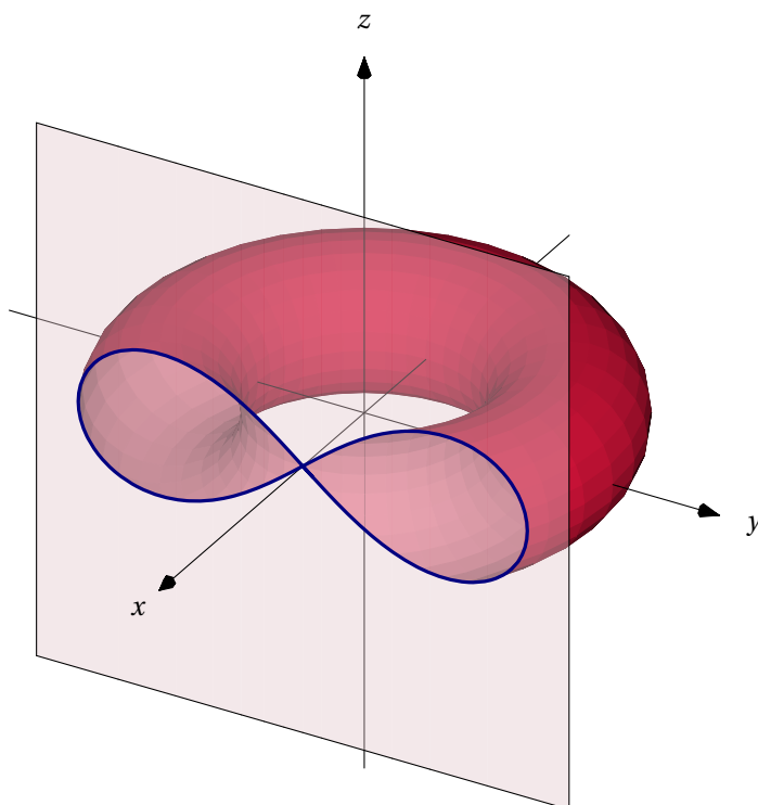
Figure 33: Torus and lemniscate
