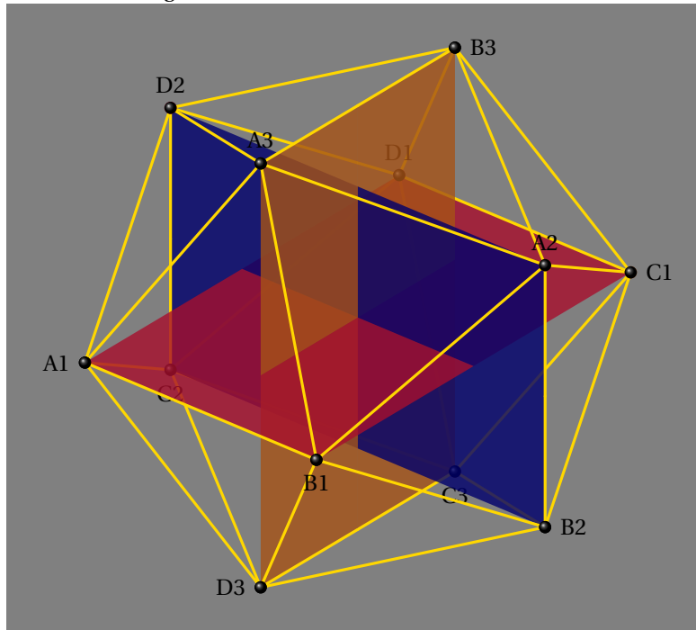
Figure 31: Construction of an icosahedron
