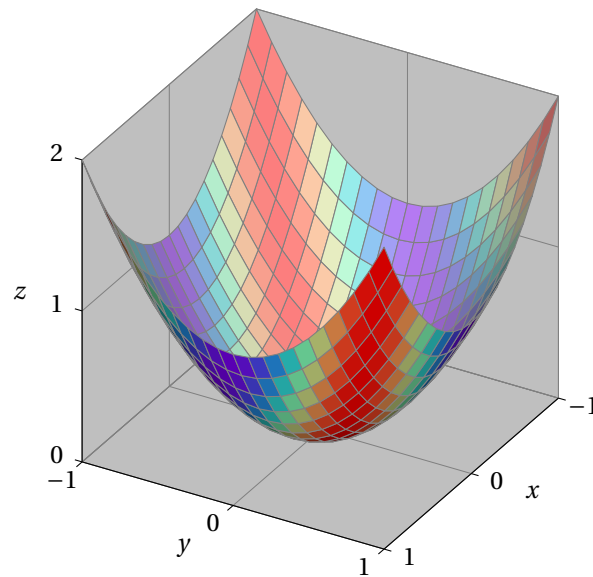
Figure 23: The function ld.read_table3d()
