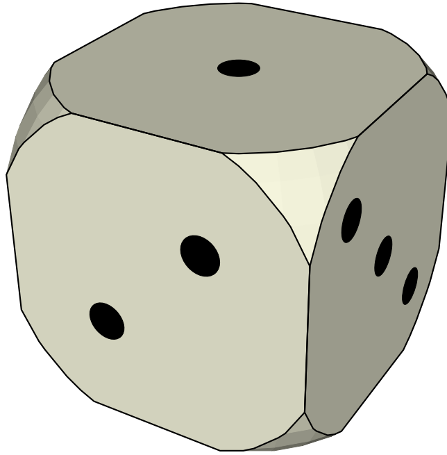
Figure 28: Example with clip3d: constructing a die from a cube and a sphere
