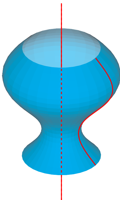
Figure 24: Example with rotcurve
