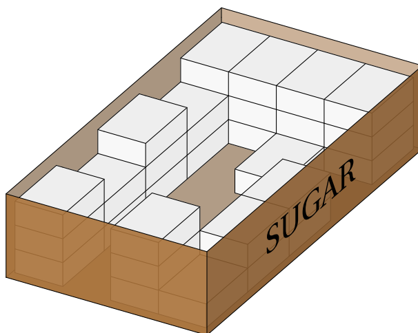
Figure 39: Box of Sugar Cubes
