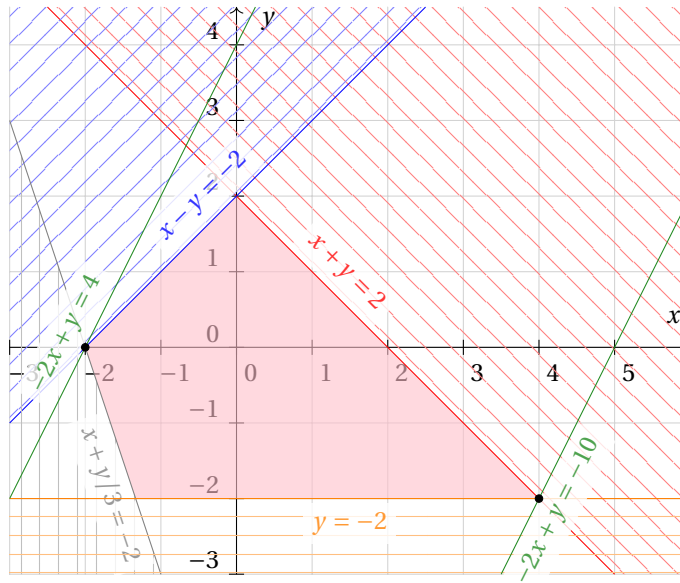
Figure 38: The g:DlinprogHalfPlanes() method
