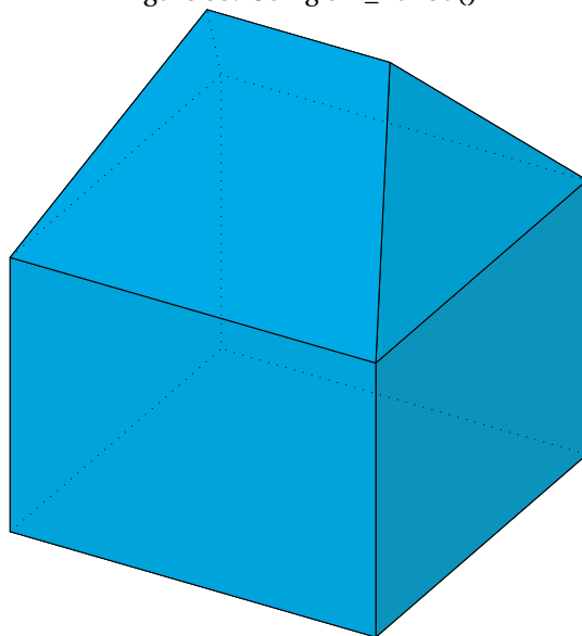
Figure 35: Using cvx_hull3d()
