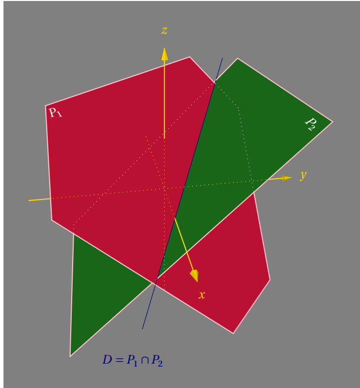
Figure 29: First example with Dscene3d: intersection of two planes
