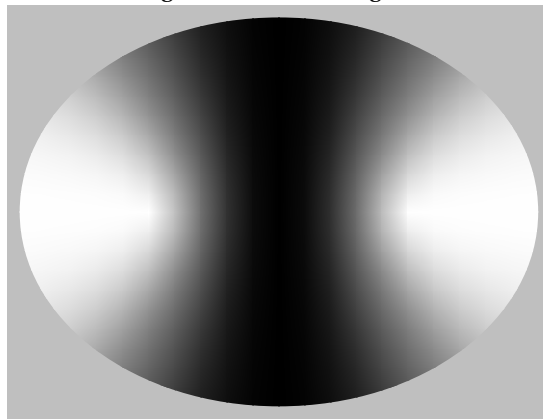
Figure 21: Shaded region
