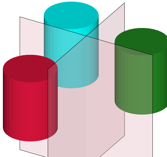
Figure 32: Example with addWall (the two transparent pink facets are normally invisible)
