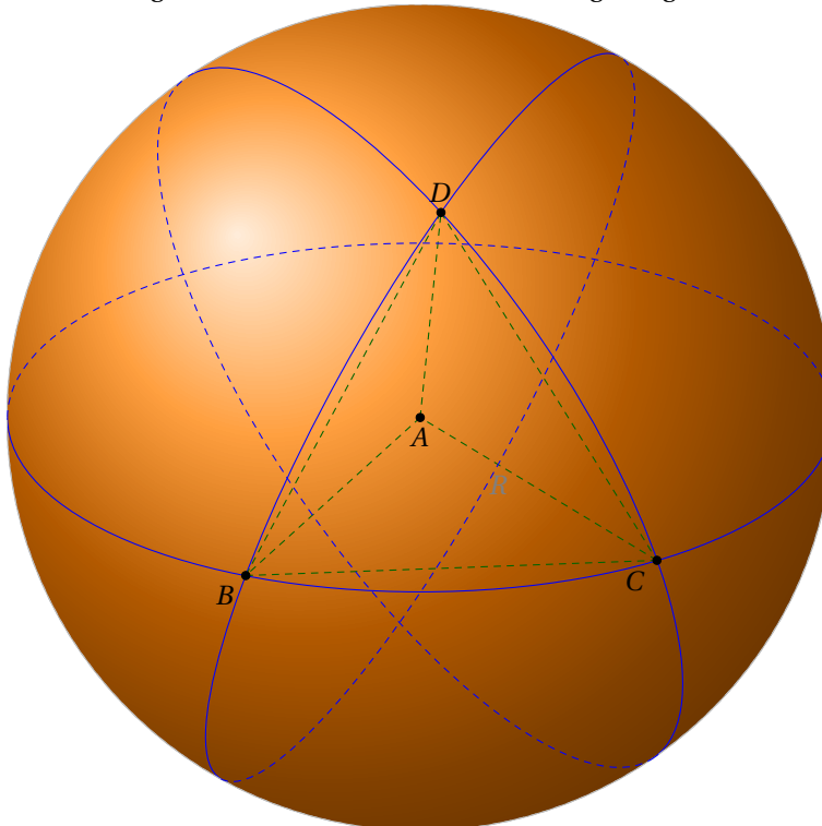
Figure 37: A tetrahedron with fixed edge lengths
