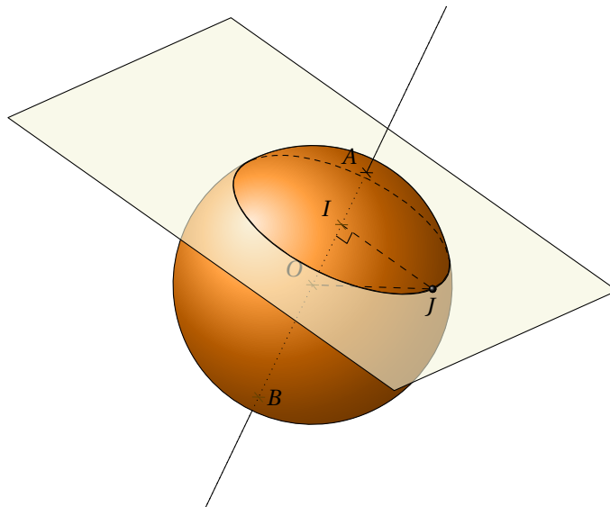
Figure 34: Section of a sphere without Dscene3d()
