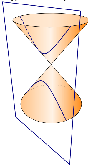
Figure 15: Hyperbola: cone-plane intersection
