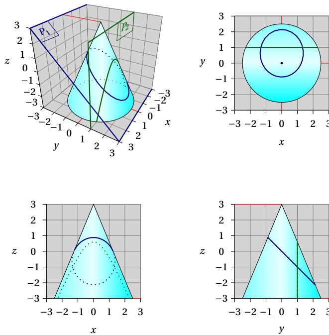
Figure 16: Cone section with multiple views
