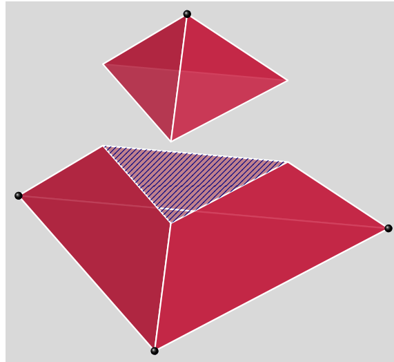
Figure 12: Section of a tetrahedron by a plane
