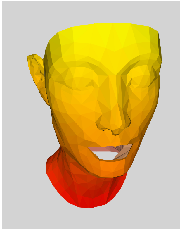
Figure 17: Mask of Nefertiti
